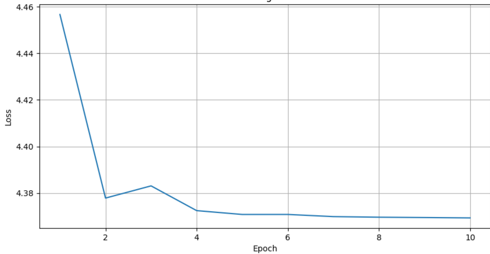
Training Loss
