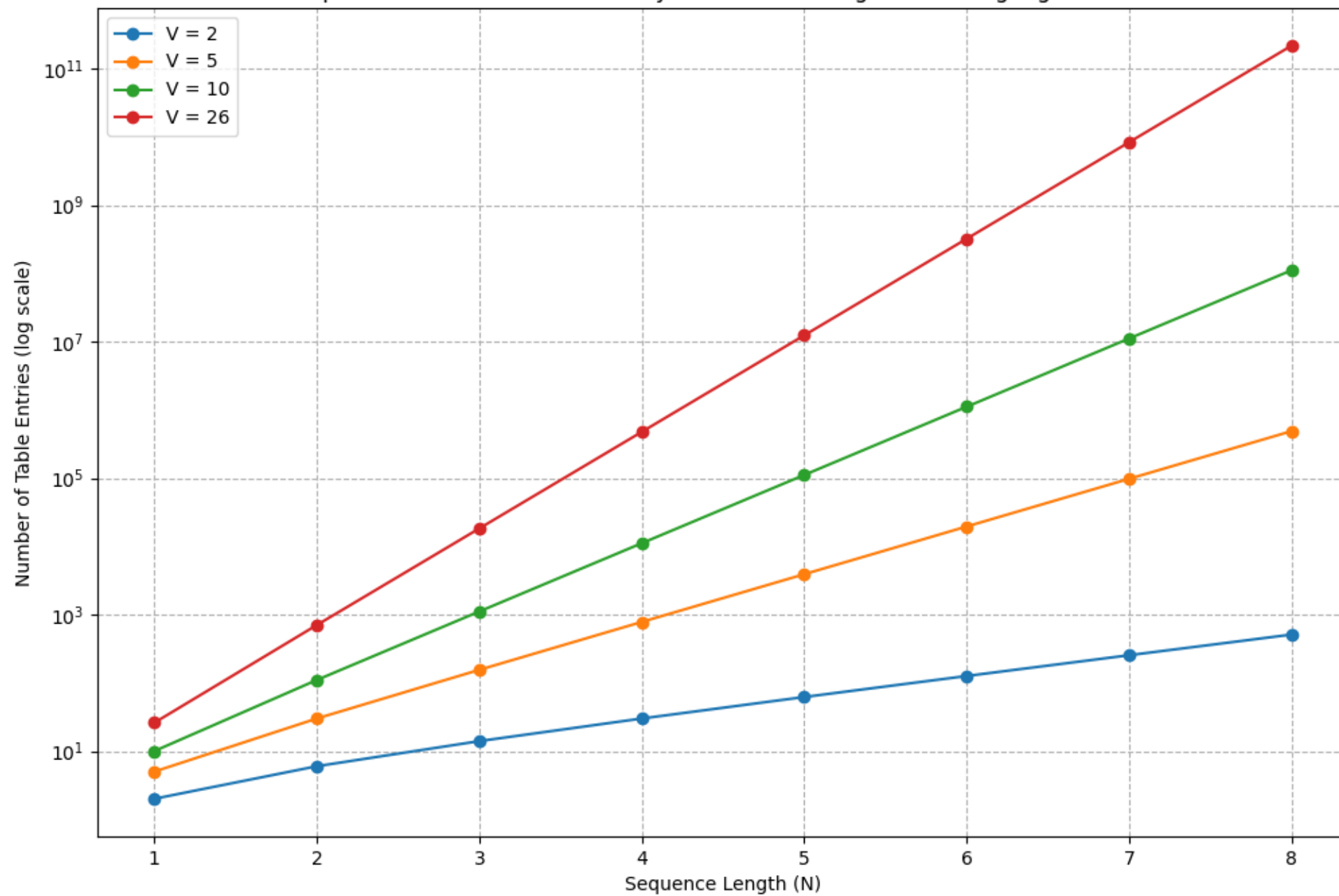
Exponential Growth of Probability Tables in Autoregressive Language Models
